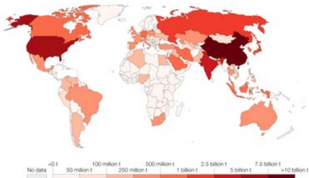
Annual CO 2 Emissions - 2019
